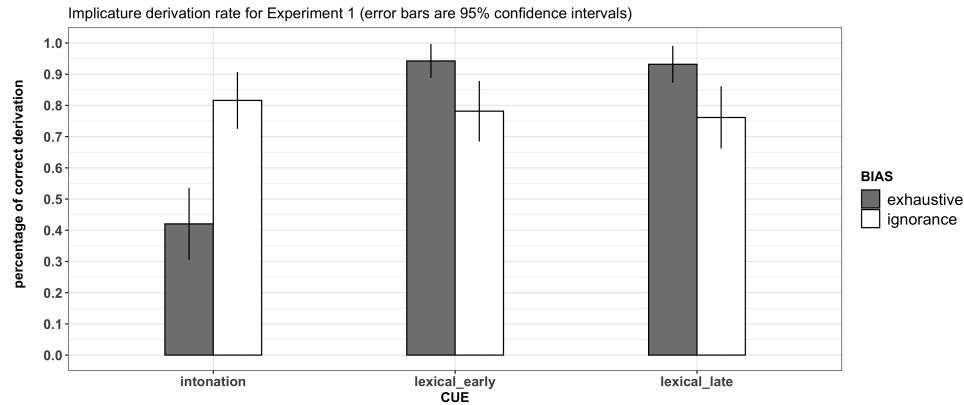
Figure 5 Implicature derivation rates for Experiment 1
